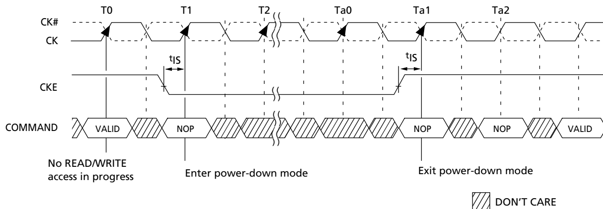
Figure 31: Power-Down
