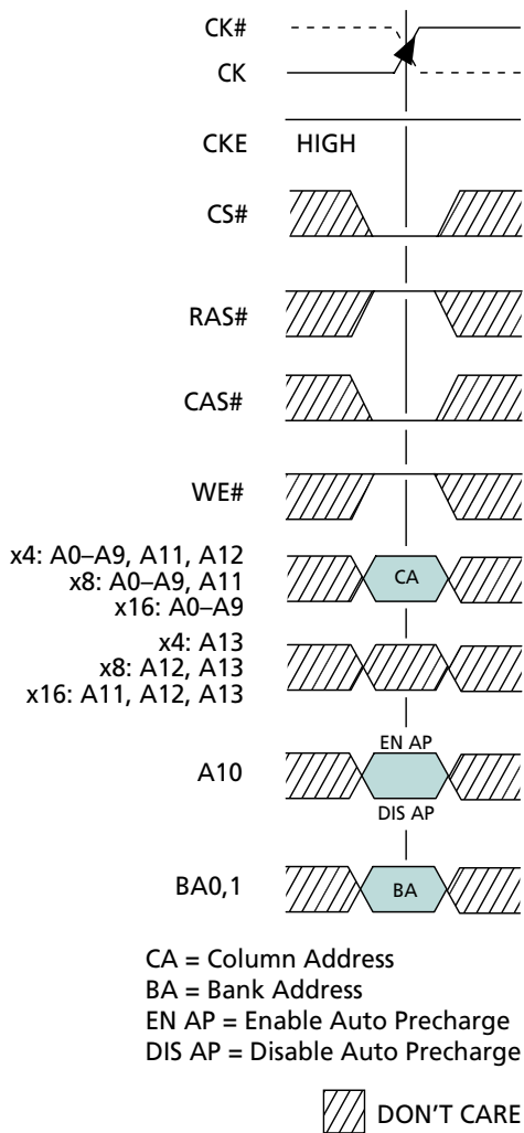
Figure 11: READ Command
