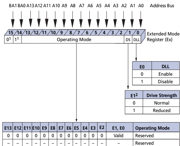
Figure 8: Extended Mode Register Definition
