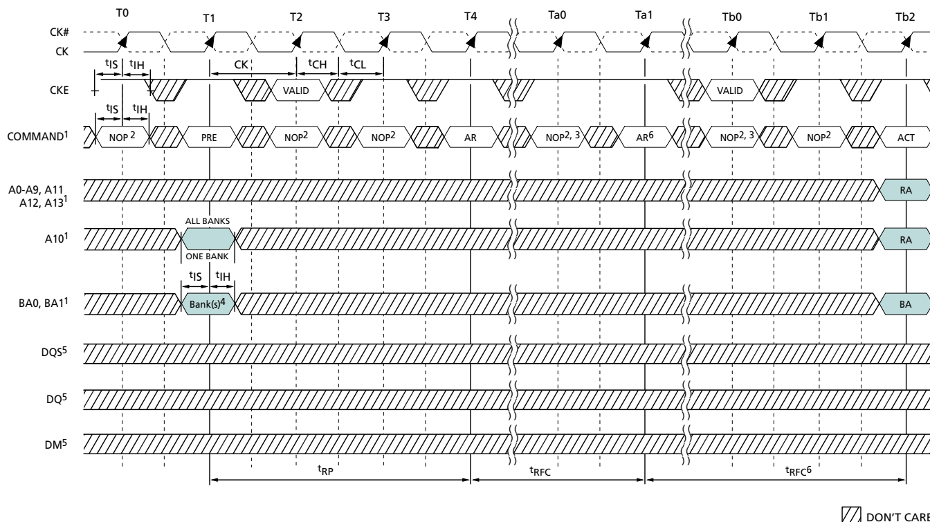
Figure 46: Auto Refresh Mode
