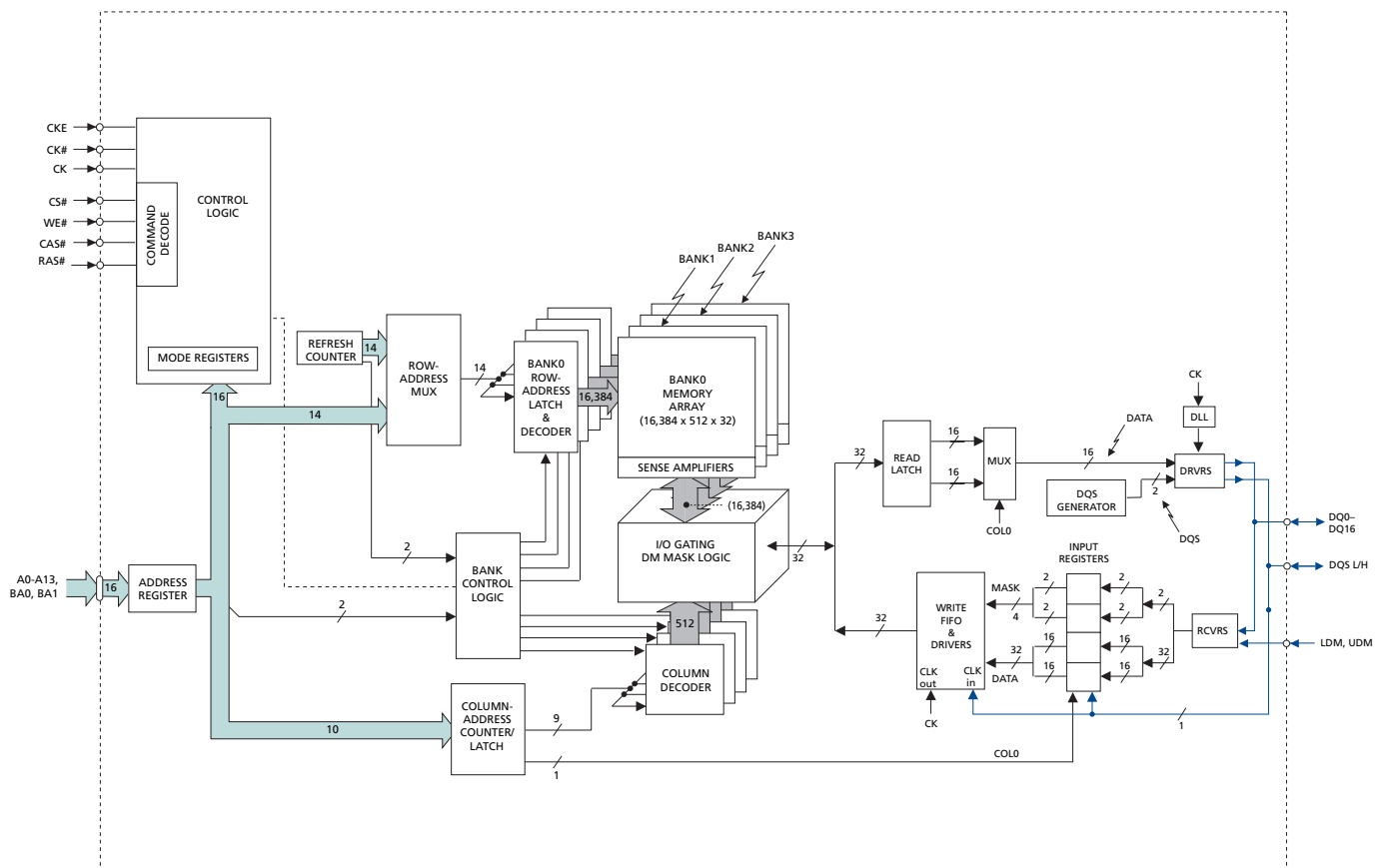
Figure 5: Functional Block Diagram 64 Meg x16
