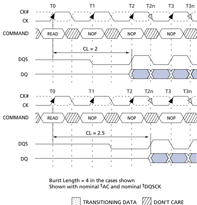
Figure 7: CAS Latency
