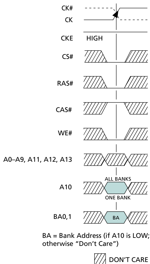
Figure 30: PRECHARGE Command
