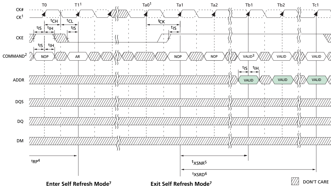
Figure 47: Self Refresh Mode
