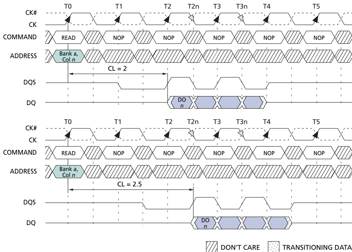
Figure 12: READ Burst
