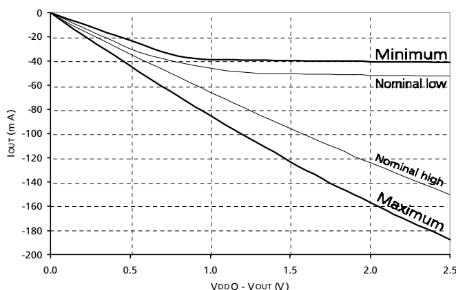
Figure 36: Full Drive Pull-Up Characteristics
