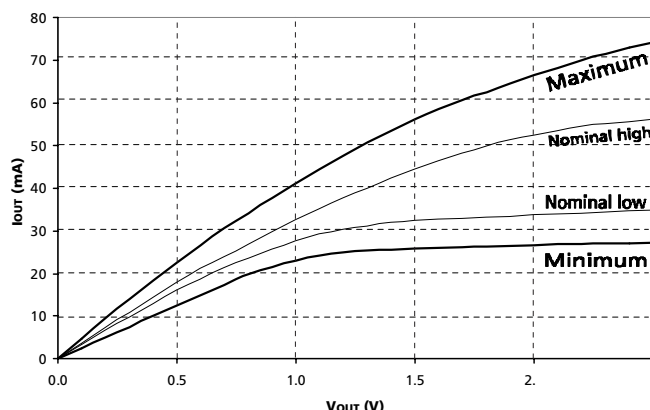
Figure 38: Reduced Drive Pull-Up Characteristics
