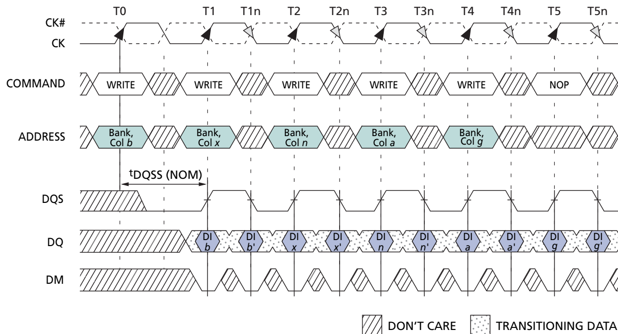
Figure 23: Random WRITE Cycles
