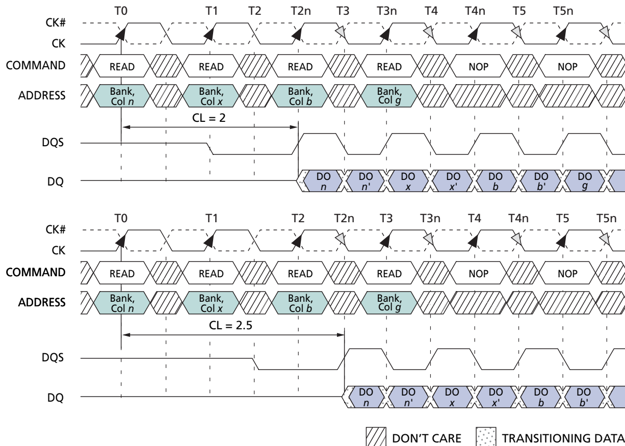
Figure 15: Random READ Accesses
