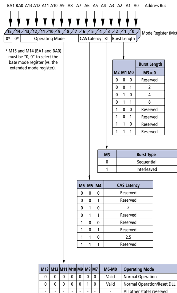
Figure 6: Mode Register Definition
